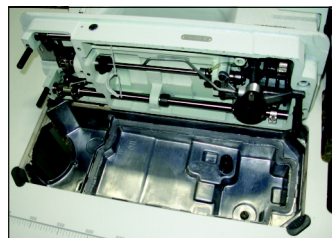
Oil Pump System with Pump, Oil Pan and Adjustable Oil Flow
